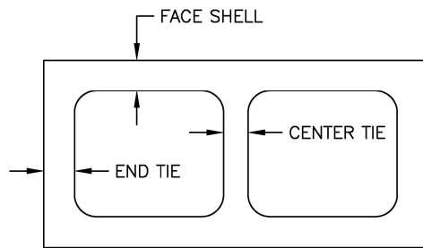
SQUARE CORE
